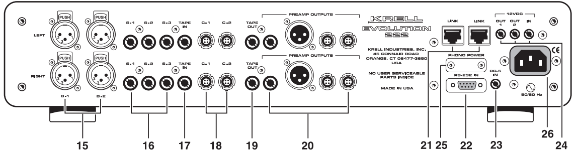
Figure 3 Evolution 222 Back Panel
